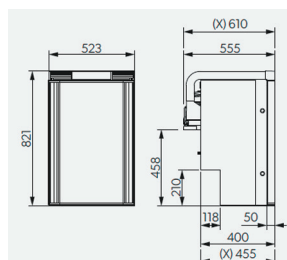
RCS 10.5XT
